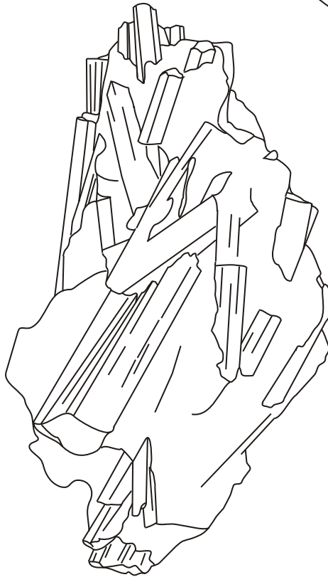
Kyanite
