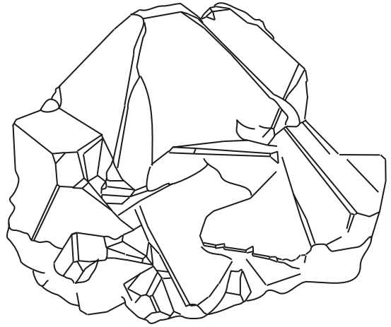
Pyrite
